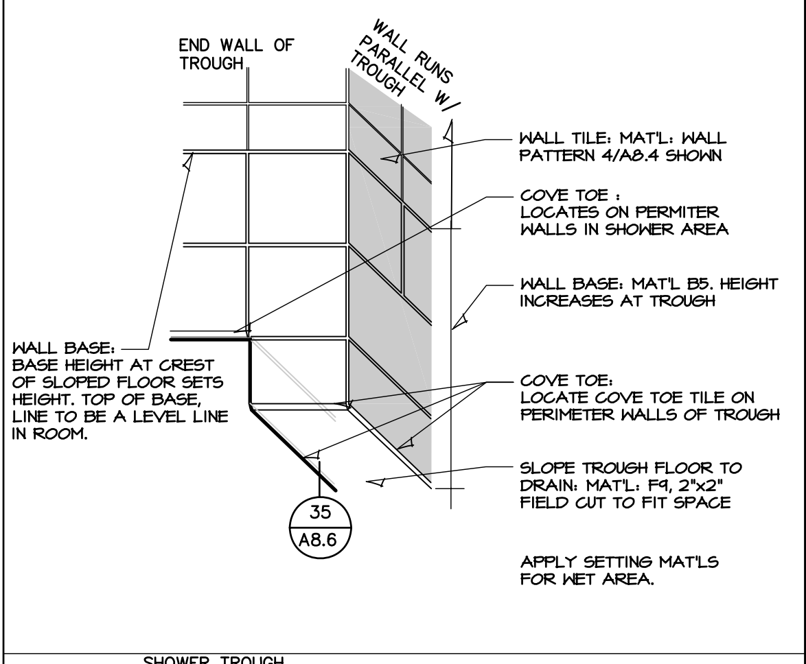
9 SHOWER TROUGH KERDI WATERPROOF MEMB. AT SHOWER REFER TO DTL 7/A8.2. MAINTAIN CURRENT TCNA INSTALL. GUIDELINES
