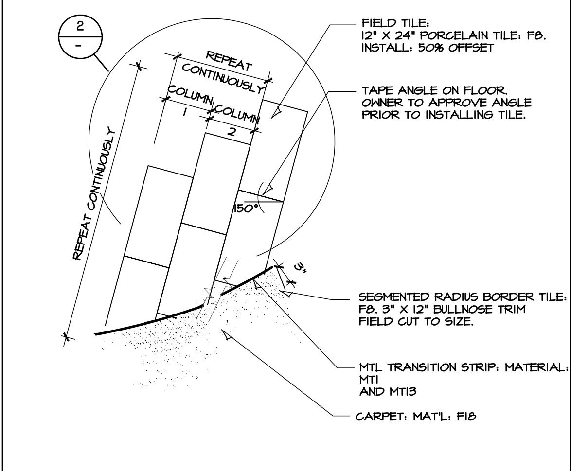
5 LOCKER ROOM ACCENT ANTI-FRACTURE MEMBRANE, TYP. REFER TO DTL 1/A8.2. MAINTAIN CURRENT TCNA INSTALL. GUIDELINES
