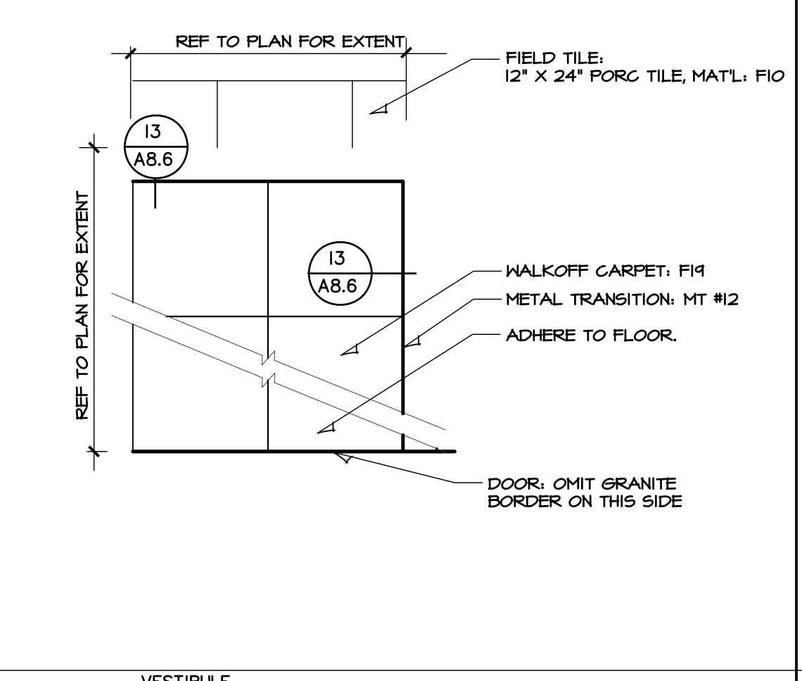
10 VESTIBULE REFER TO DTL 5/A8.2. MAINTAIN CURRENT TCNA INSTALL. GUIDELINES
