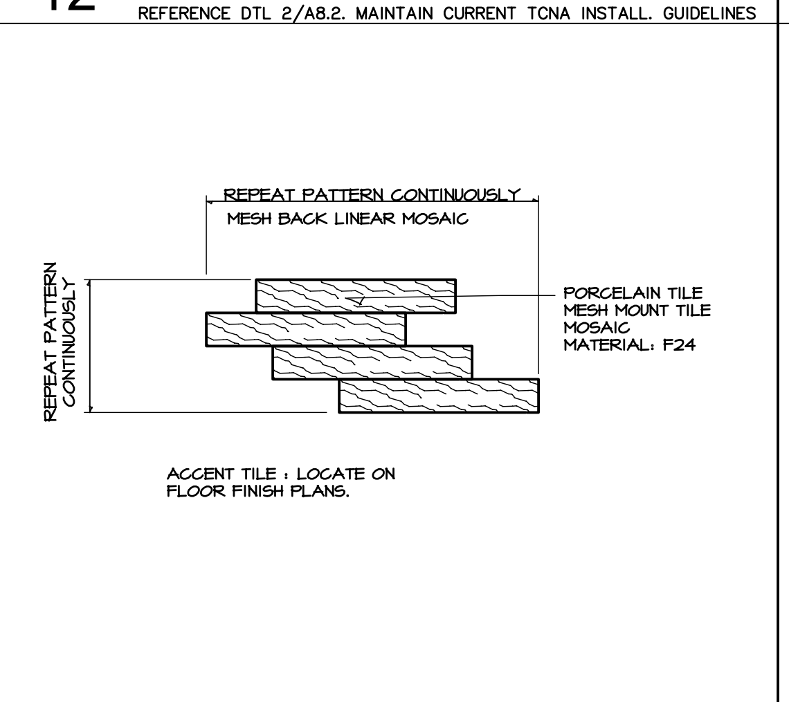
15 TILE BORDER ANTI-FRACTURE MEMBRANE, TYP. REFER TO DTL 5/A8.2. MAINTAIN CURRENT TCNA INSTALL. GUIDELINES
