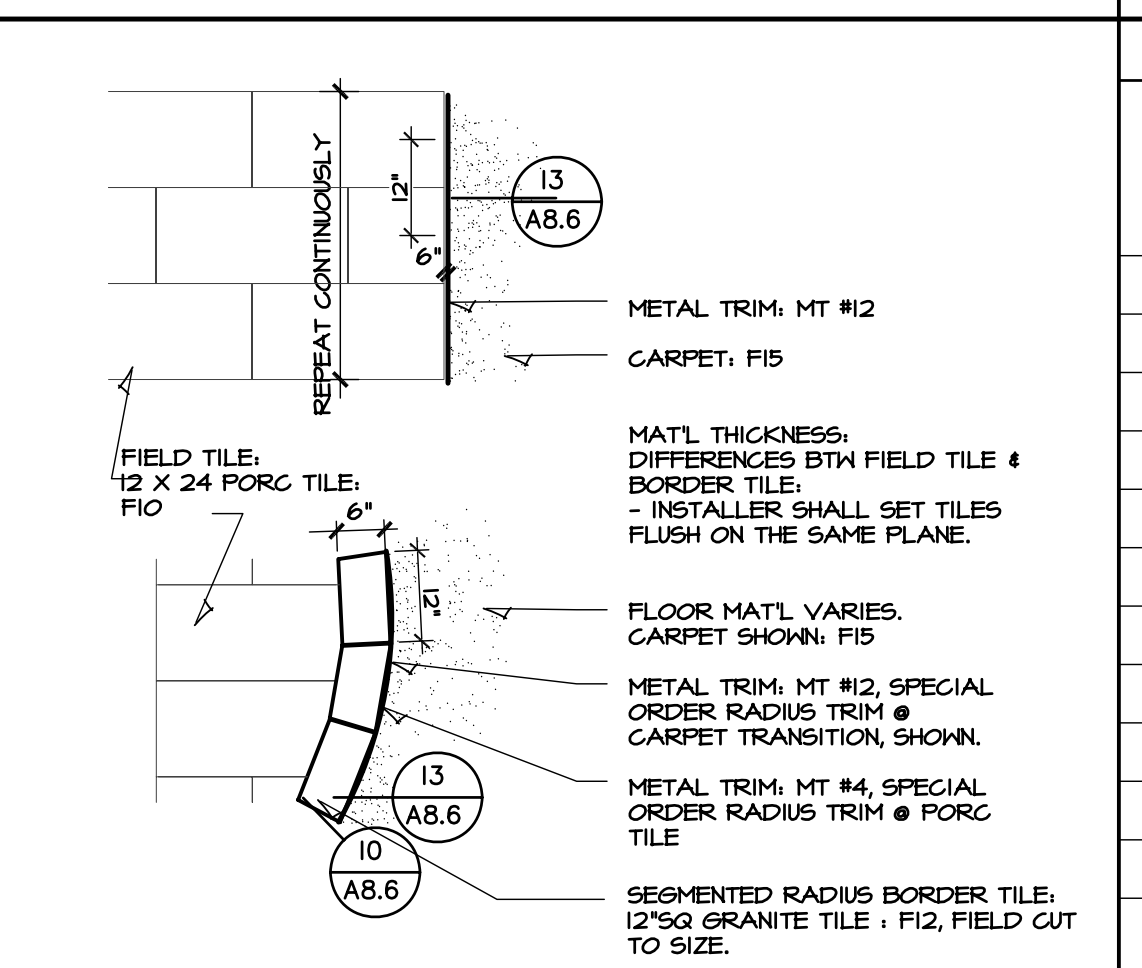
4 TILE BORDER ANTI-FRACTURE MEMBRANE, TYP. REF TO DTL 5/A8.2. MAINTAIN CURRENT TCNA INSTALL. GUIDELINES
