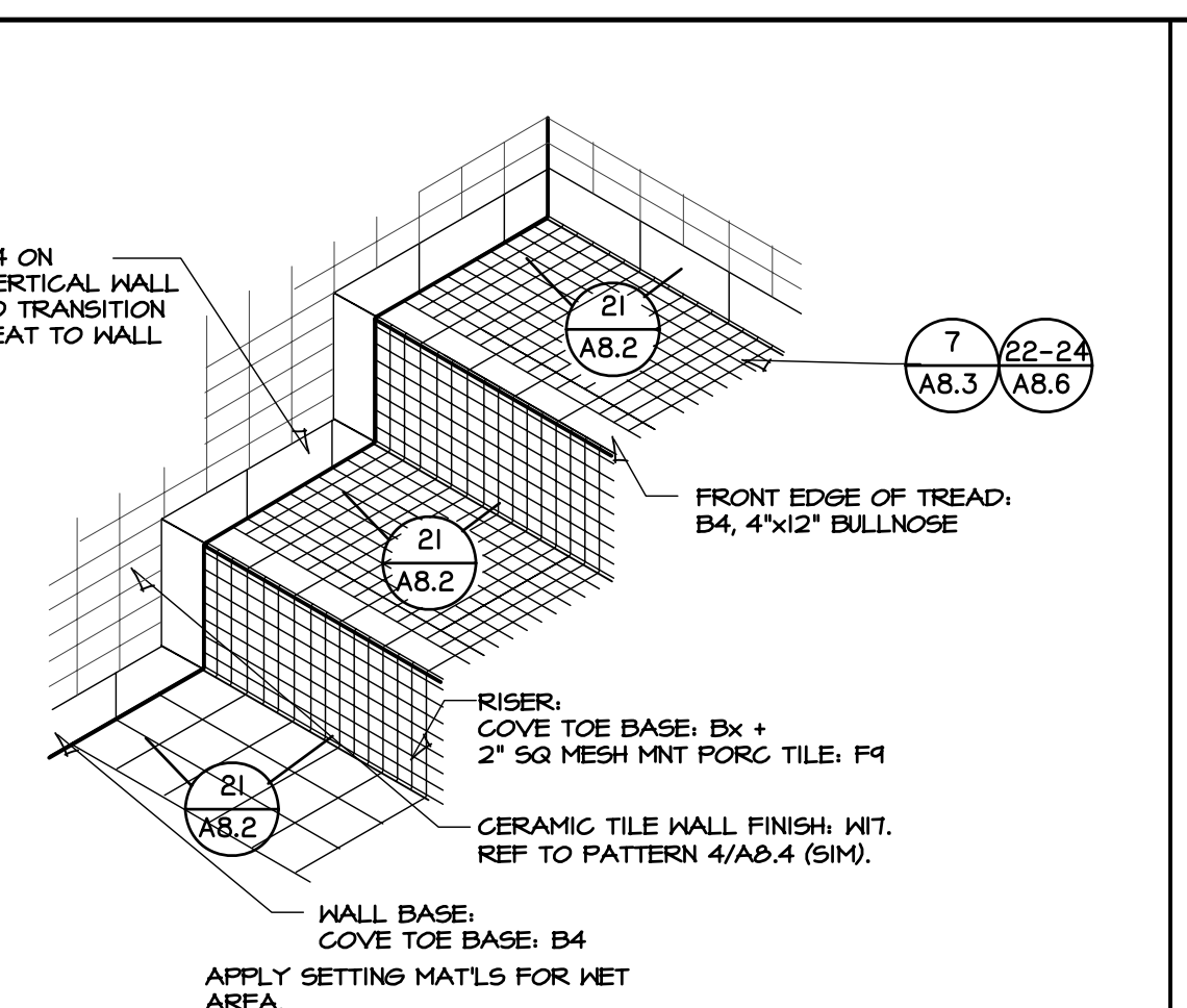
3 STEAM ROOM RISERS KERDI DS WATERPROOF MEMBRANE, REFER TO DTL 6/A8.2AT RISERS. REFER TO DTL 8/A8.0. MAINTAIN CURRENT TCNA INSTALL. GUIDELINES
