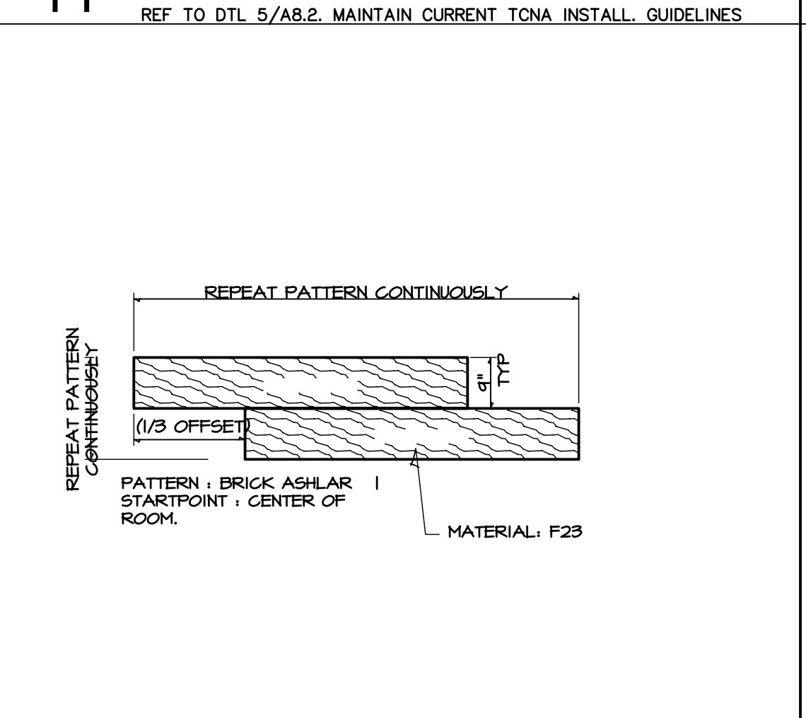
14 LUXURY VINYL PLANKS MEMBRANE CRACK ISOLATION, FULL COVERAGE ADHESIVE DIRECT GLUE, DOUBLE STICK
