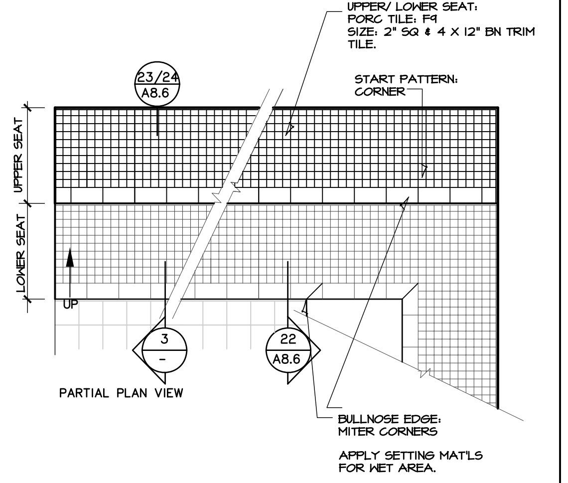
7 STEAM ROOM RISER CORNER KERDI DS WATERPROOF MEMBRANE REFER TO DTL 6/A8.0 AT RISERS. REFER TO DTL 8/A8.2. MAINTAIN CURRENT TCNA INSTALL. GUIDELINES
